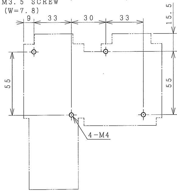
MOUNTING HOLES.
