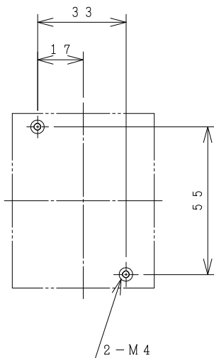
MOUNTING HOLES.
