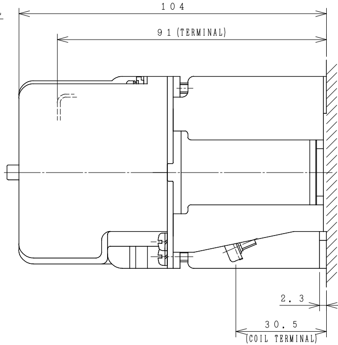
OUTLINE DIMENSIONS.
