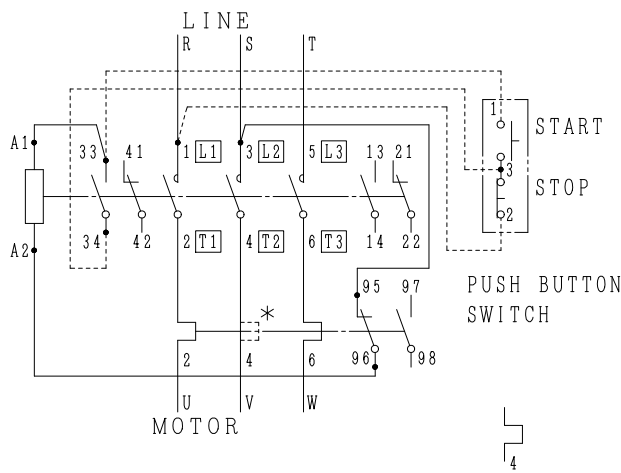
CONTACTS ARRANGEMENT.
