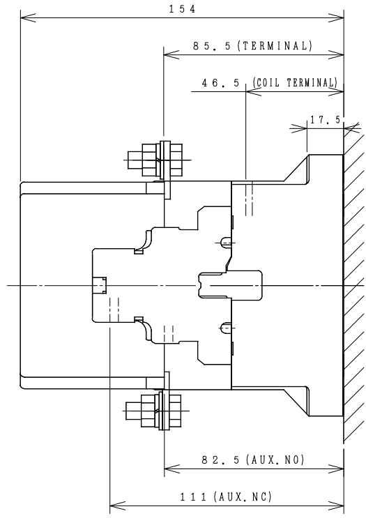
OUTLINE DIMENSIONS.
