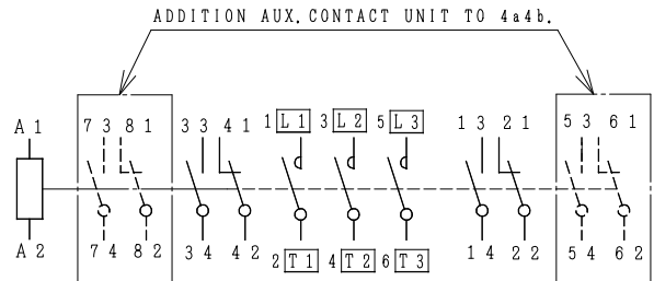
CONTACTS ARRANGEMENT.
