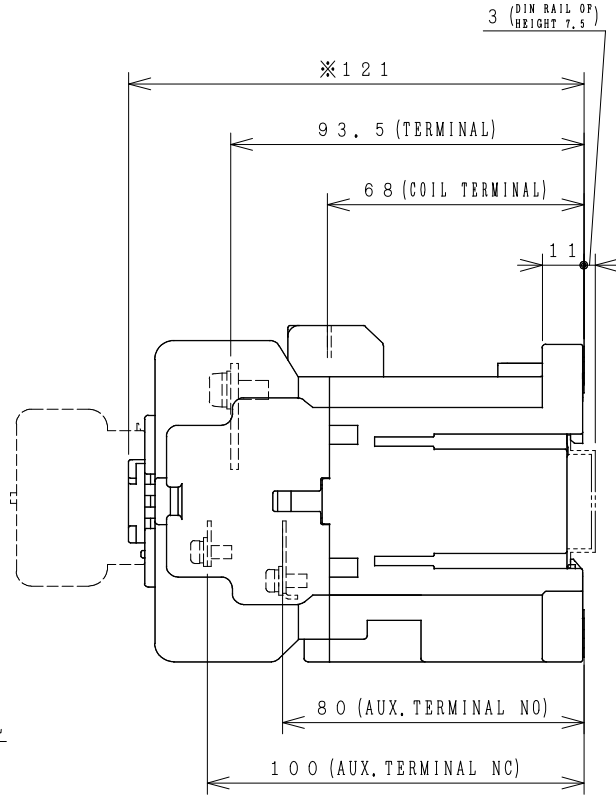
OUTLINE DIMENSIONS.
