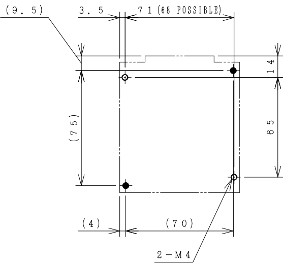
MOUNTING HOLES.
