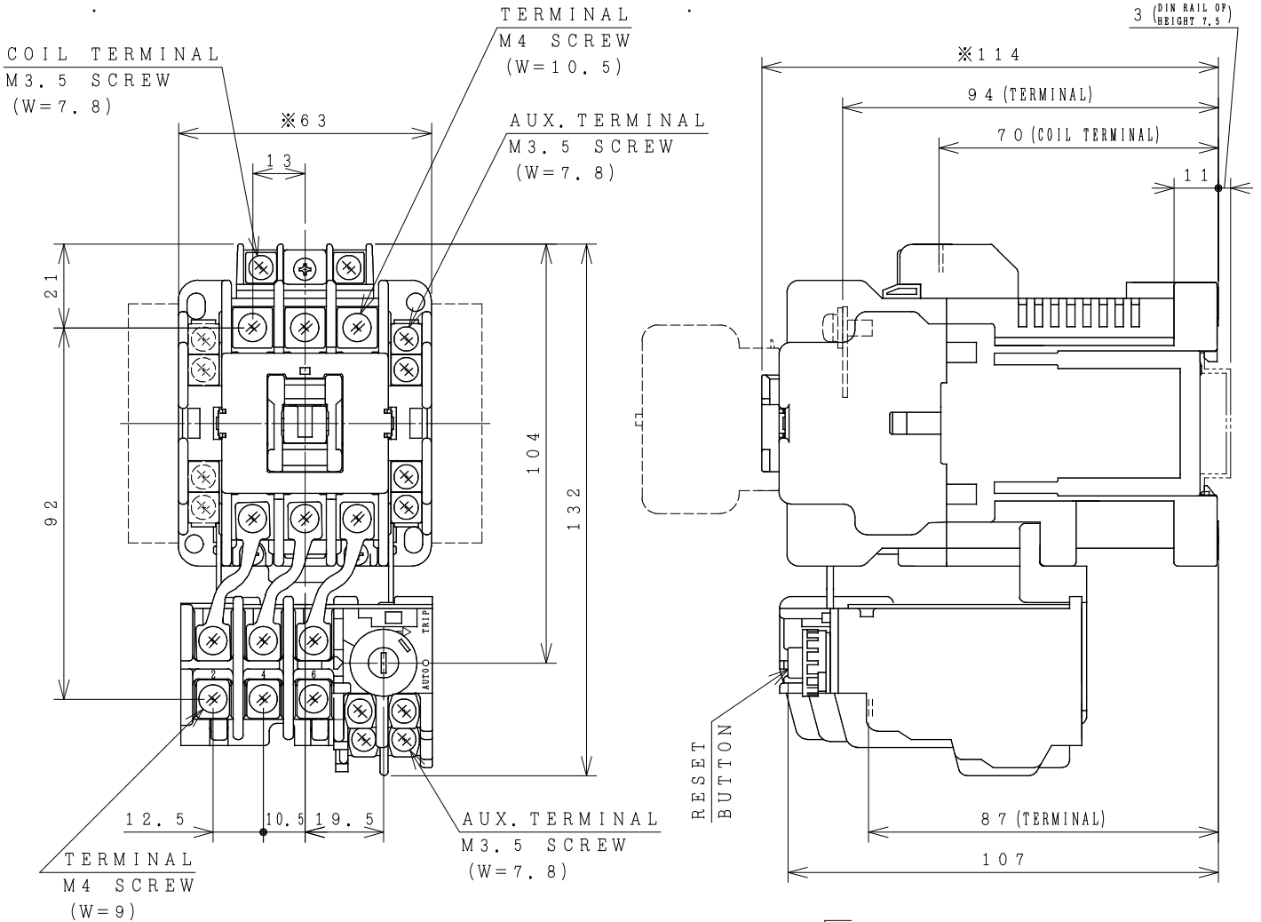
OUTLINE DIMENSIONS.
