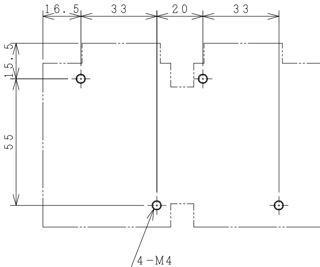
MOUNTING HOLES.
