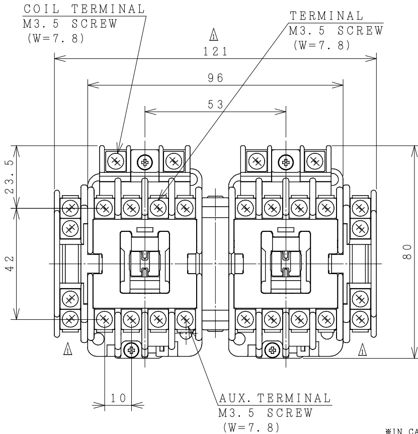
OUTLINE DIMENSIONS.
