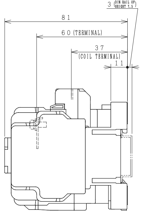
OUTLINE DIMENSIONS.
