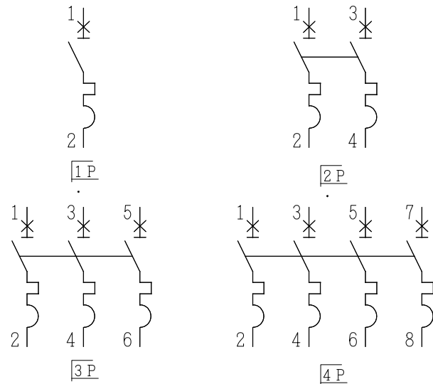
WIRING DIAGRAM
