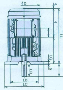
Shaft Dimension
