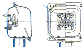
Illustration of outside wire connection
